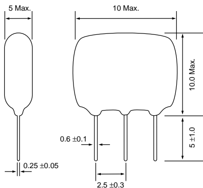
Figure 3) ZTT □.□□MT, MX Front and Side views
